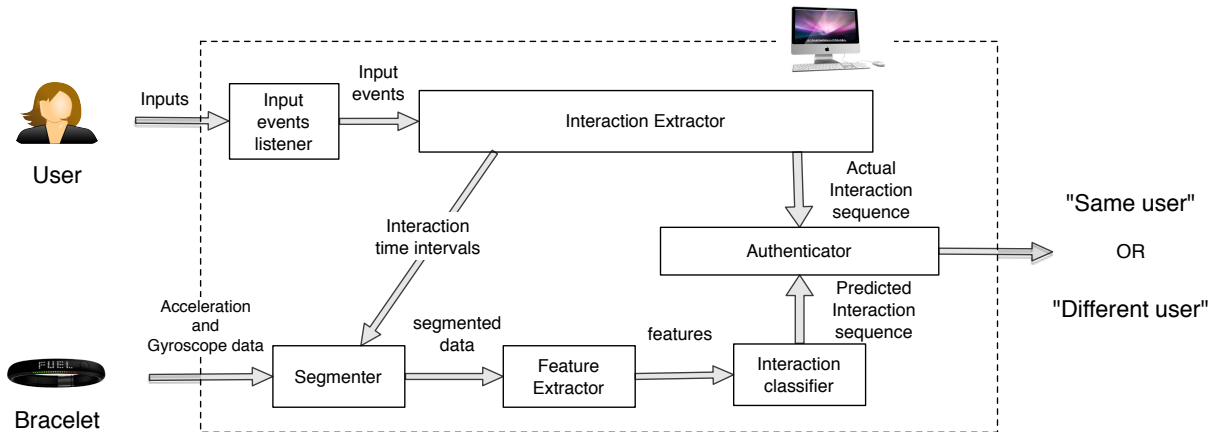
Figure 2: ZEBRA architecture.
