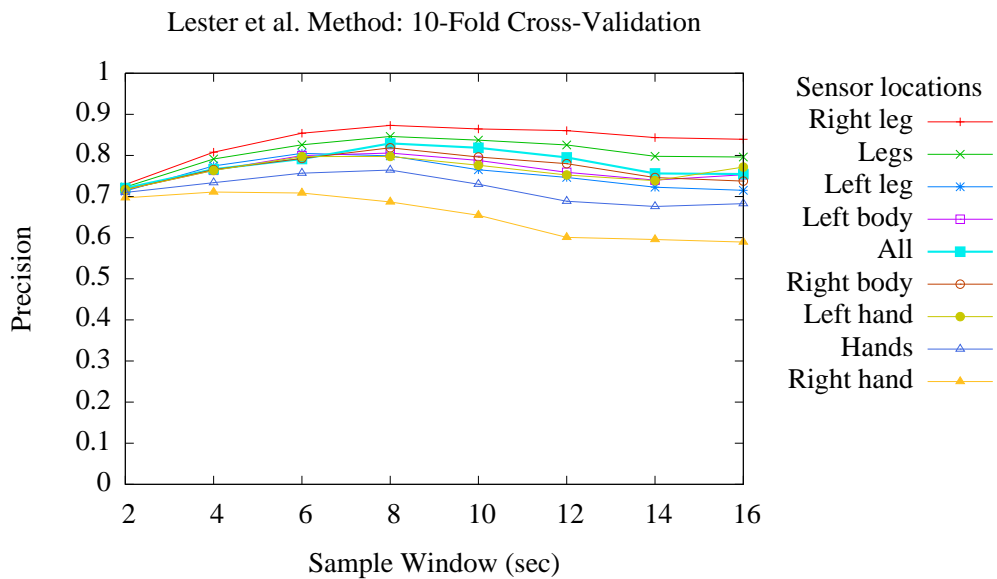
Figure 7: A 10-fold cross-validation of the Lester et al. method. Precision was computed across all users for each of the specified locations while varying the coherence window.
