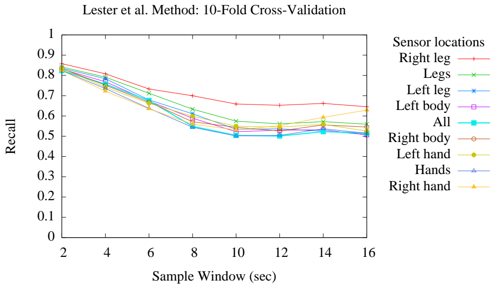
Figure 8: A 10-fold cross-validation of the Lester et al. method. Recall was computed across all users for each of the specified locations while varying the coherence window.
