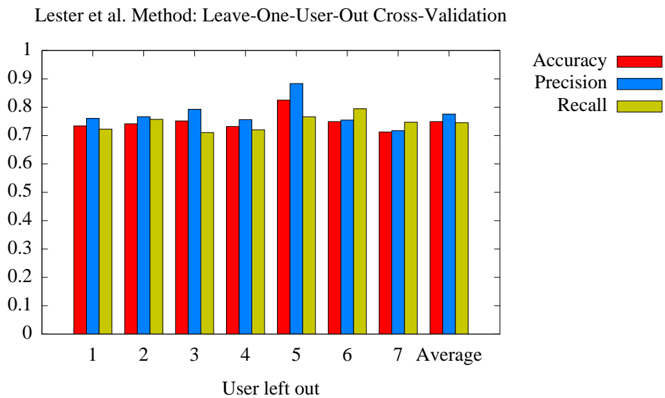
Figure 9: A leave-one-user-out validation of the Lester et al. method for each user as well as the average across all users. The coherence window was fixed to 4 seconds as this yielded the best results.
