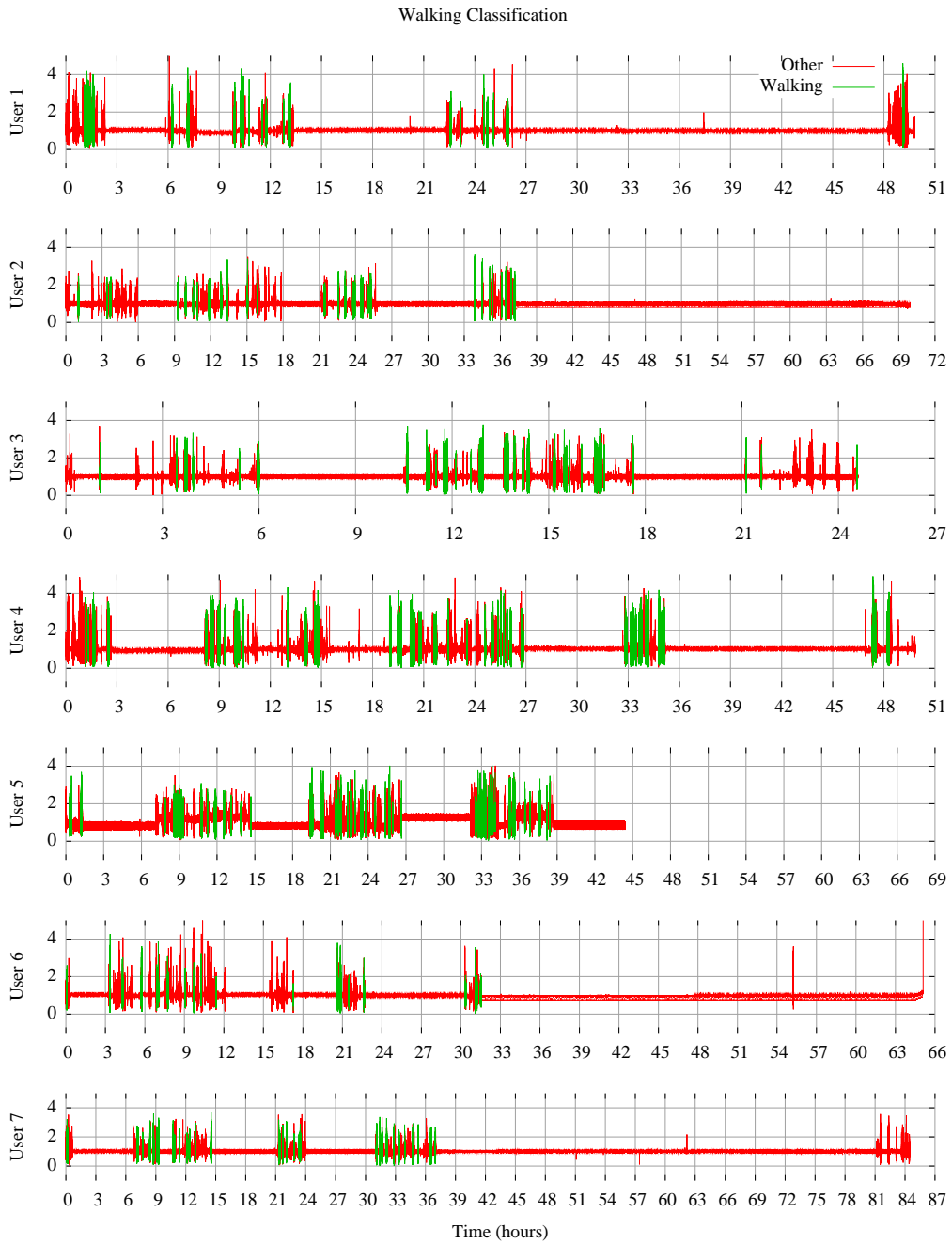
Figure 11: Walking classification for each user for the whole time that they carried the sensor. According to the classification method, users walked for 74 seconds on average and in total walked an average of 2.3% (1.9% aggregated) of the collection period.
