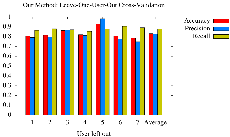
Figure 5: A leave-one-user-out validation of our method for each user as well as the average across all users. The coherence window was 8 seconds as this yielded the best results.
