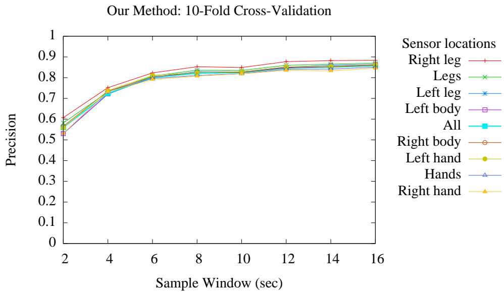
Figure 3: A 10-fold cross-validation of our method. Precision was computed across all users for each of the specified locations while varying the coherence windows. The feature window was fixed to 17 samples as this yielded the best results.
