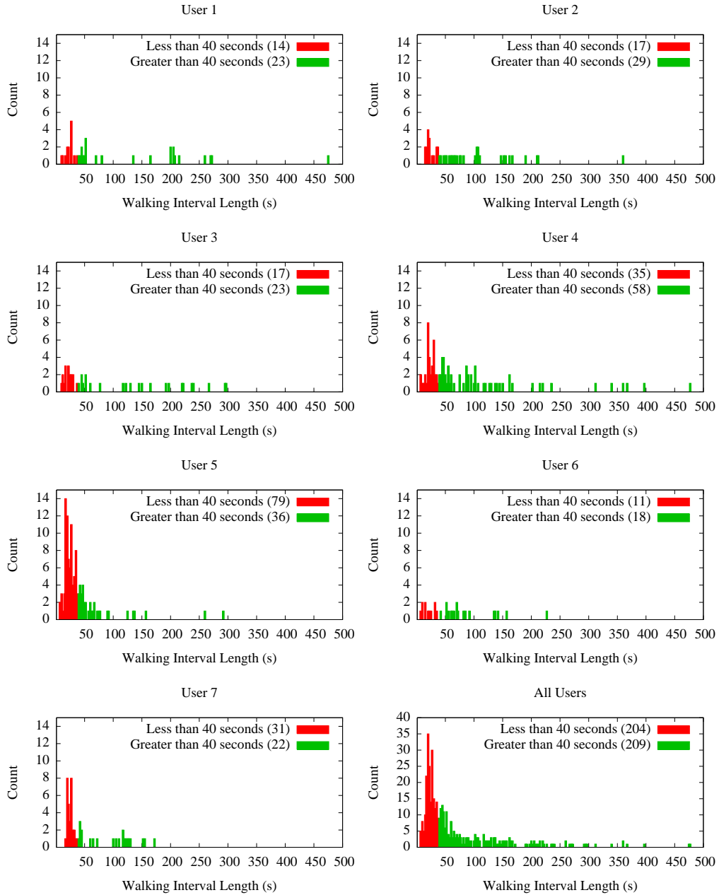
Figure 12: The distribution of walking interval lengths for all users and the aggregation of all users. Features were extracted every 5 seconds with 50% overlap. The aggregated distribution tends to skew heavily towards shorter walking intervals for this particular set of users.
