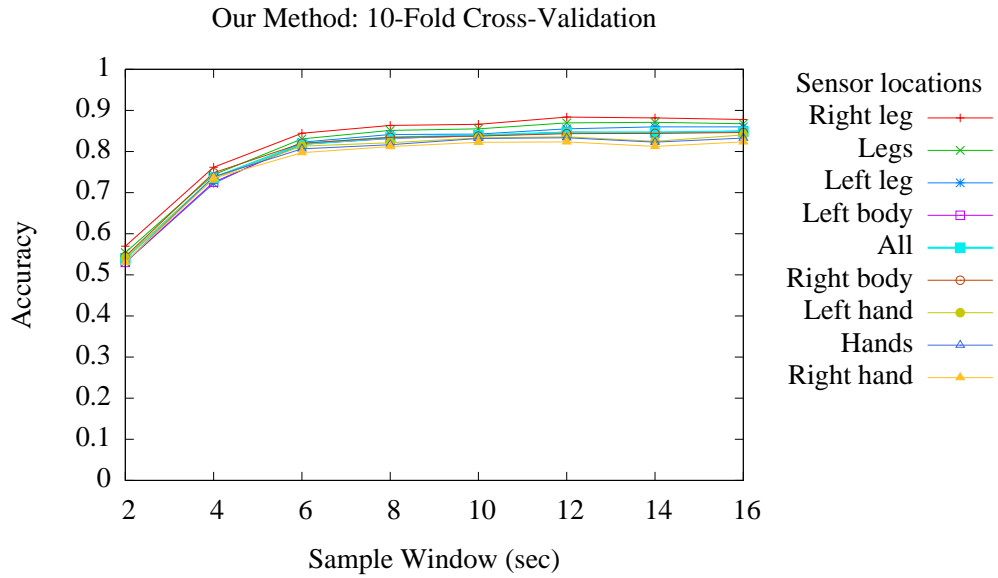
Figure 2: A 10-fold cross-validation of our method. Accuracy was computed across all users for each of the specified locations while varying the coherence windows. The feature window was fixed to 17 samples as this yielded the best results.
