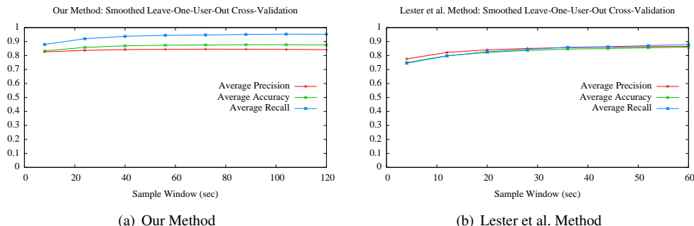
Figure 10: A smoothed leave-one-user-out cross-validation of the specified method. Average accuracy, precision and recall was computed by varying the smoothing window and averaging across all users. The coherence window was fixed to 8 seconds for our method and 4 seconds for the Lester et al. method as this yielded the best results.
